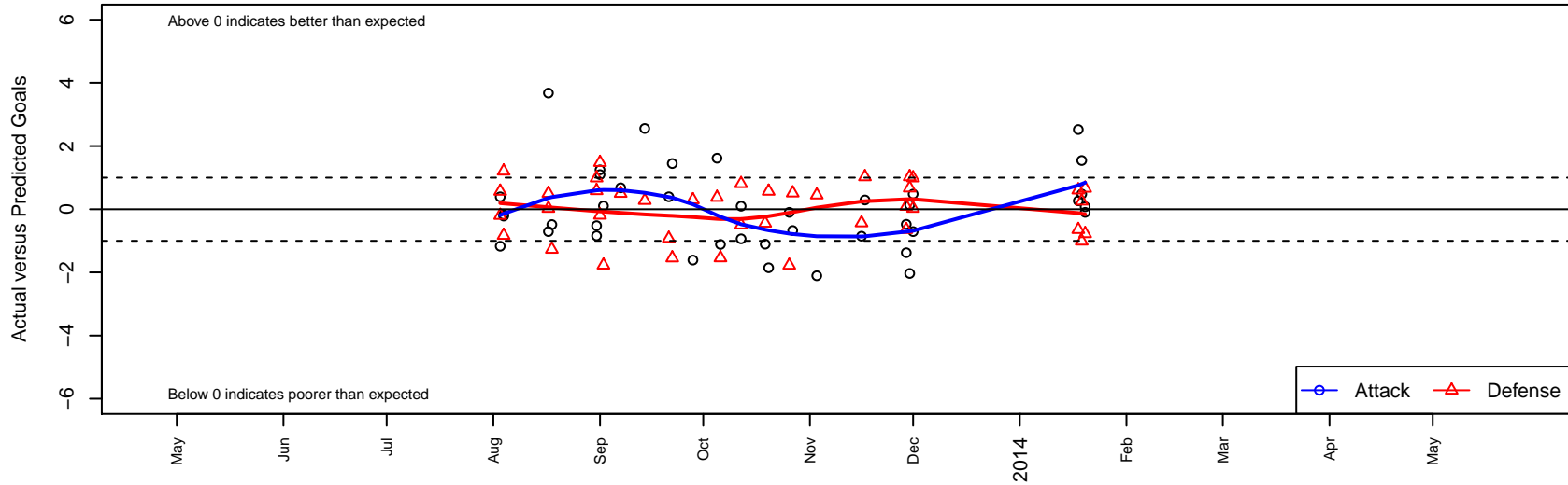
Beach FC Black G00 Dots are actual minus expected GF (blue circles) and GA (red triangles). Blue line is smoothed change in attack strength. Red is smoothed change in defense strength.
